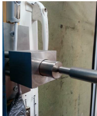
Cutting test block and restrictor mounted in test rig
