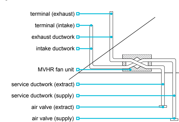
Figure 1: MVHR schematic
