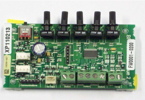
XP110213 'A' & 'ABD' Control PCB
