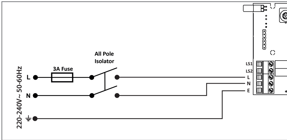
Supply Wiring Diagram 220-240V~ 50-60Hz ref EE 184
