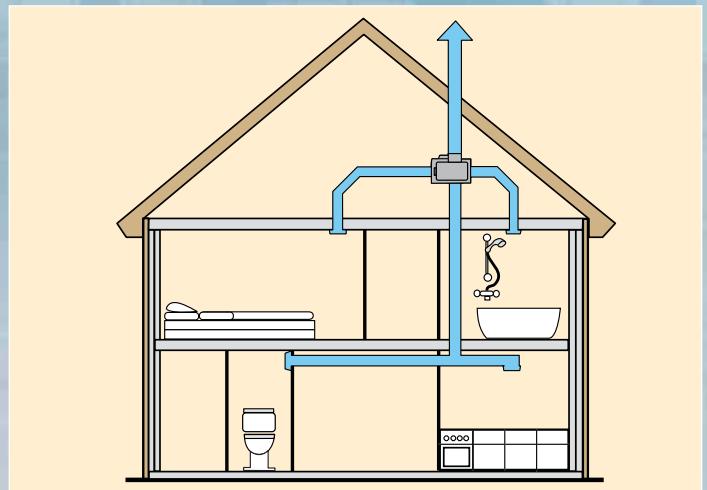
MVS-8 typical application
